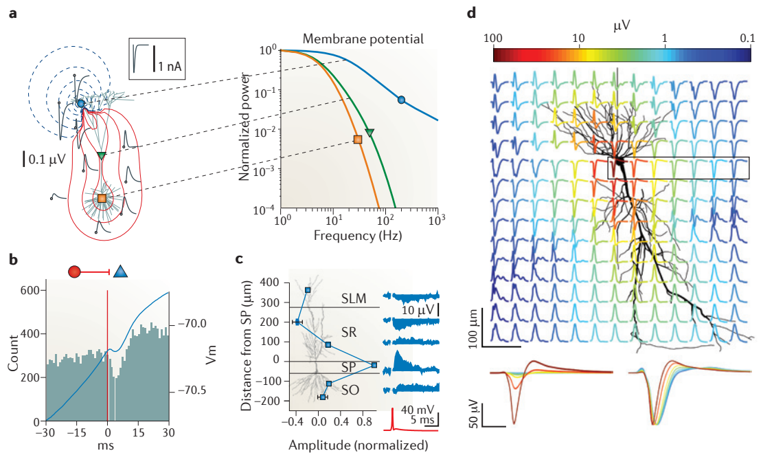
Figure 2 | Excitatory and inhibitory postsynaptic currents are the most ubiquitous contributors to V_e . a | Computer-simulated local field potential (LFP) traces (left panel; grey) in response to an excitatory synaptic current input (a sink, shown by the blue circle) injected into the distal apical dendrite of a purely passive layer 5 pyramidal model neuron. The waveform of the injected current is illustrated in the box. Red and blue contour lines correspond to positive and negative values for the LFP amplitude, respectively. The calculated double logarithmic power spectra of the transmembrane potential are also shown (right panel), following injection of current into the apical dendrite near the injection site (blue trace), mid-apical dendrite (green trace) and soma (orange trace). Note that high-frequency activity decreases with the distance from the active synaptic site (that is, the sink). b | A monosynaptic inhibitory connection between a putative layer 3 entorhinal cortical interneuron (red circle) and intracellularly recorded pyramidal cell (blue triangle). Below it, a cross-correlogram between the spikes of the reference interneuron (at time 0, red line) and the pyramidal cell and, superimposed on it, the spike-triggered average of the membrane potential ( V_m ) of the pyramidal cell (in blue). Note the small, short-latency hyperpolarization (the dip) superimposed on the rising phase of the intracellular theta oscillation and the corresponding decreased spike discharge of the pyramidal cell. c | Inhibition-induced LFPs were generated in the vicinity of a pyramidal neuron (bottom cell) by intracellularly induced action potentials in a nearby basket cell (top cell), and were recorded extracellularly at six sites in multiple layers of the hippocampus. The mean LFP amplitude at each site is shown by the blue squares. Example LFP traces (blue) from six sites and the action potential of the basket cell (red trace) are shown on the right. Note that the largest positive response by inhibition-induced hyperpolarization occurs near the soma. d | Extracellular contribution of an action potential ('spike') to the LFP in the vicinity of the spiking pyramidal cell. The magnitude of the spike is normalized. The peak-to-peak voltage range is indicated by the colour of the traces. Note that the spike amplitude decreases rapidly with distance from the soma, without a change in polarity within the pyramidal layer (the approximate area of which is shown by the box), in contrast to the quadrupole (that is, reversed polarity signals both above and below the pyramidal layers) formed along the somatodendritic axis. The distance-dependence of the spike amplitude within the pyramidal layer is shown (bottom left panel) with voltages drawn to scale, using the same colour identity as the traces in the boxed area in d . The same traces are shown normalized to the negative peak (bottom right panel). Note the widening of the spike with distance from the soma, owing to greater contributions from dendritic currents and intrinsic filtering of high-frequency currents by the cell membrane. SLM, stratum lacunosum moleculare; SO, stratum oriens; SP, stratum pyramidale; SR, stratum radiatum. Part a is reproduced, with permission, from REF. 83 © (2010) Springer. Part b is reproduced, with permission, from REF. 137 © (2010) Society for Neuroscience. Part c is reproduced from REF. 29 © (2009) Macmillan Publishers Ltd. All rights reserved. Part d courtesy of E. W. Schomburg, California Institute of Technology, USA.
